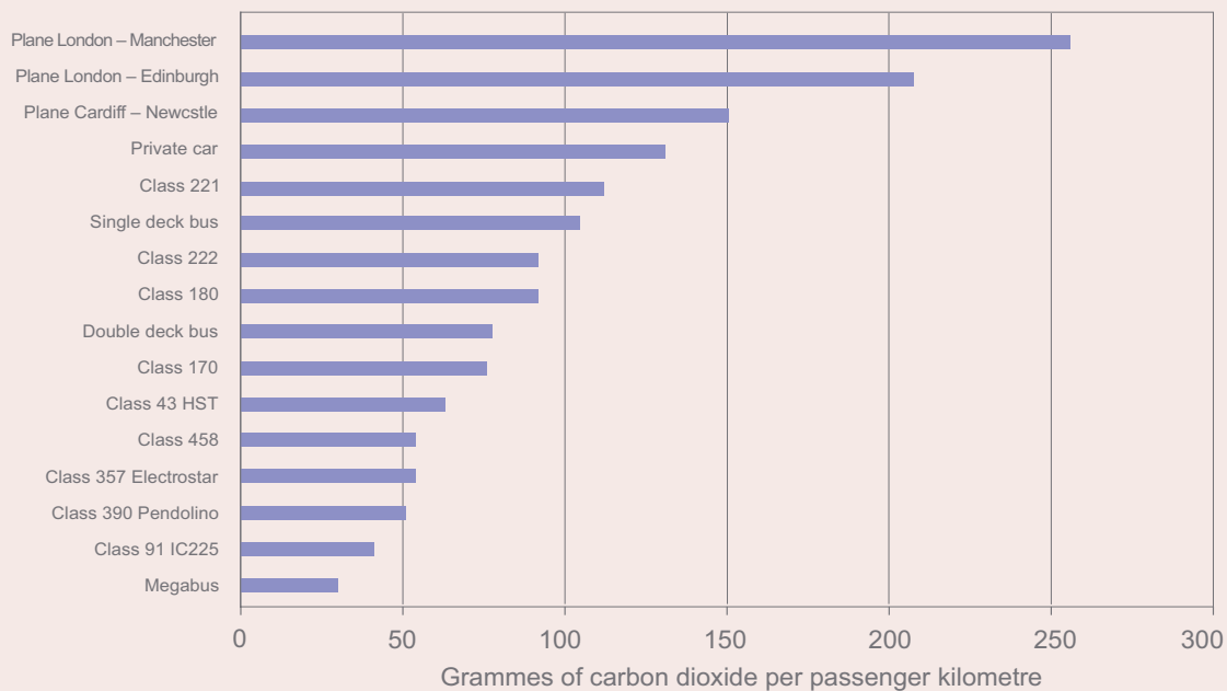
Figure 4.3 – Relative carbon performance of rail and other modes
