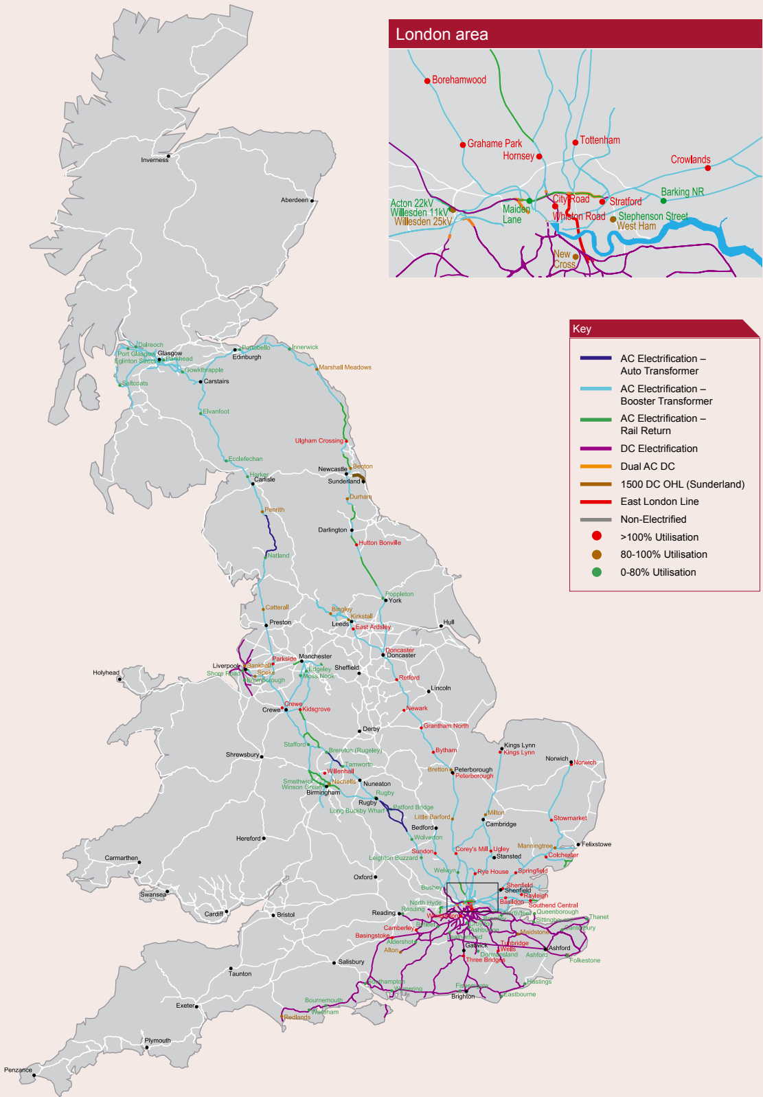
Figure 3.8 – Power supply
