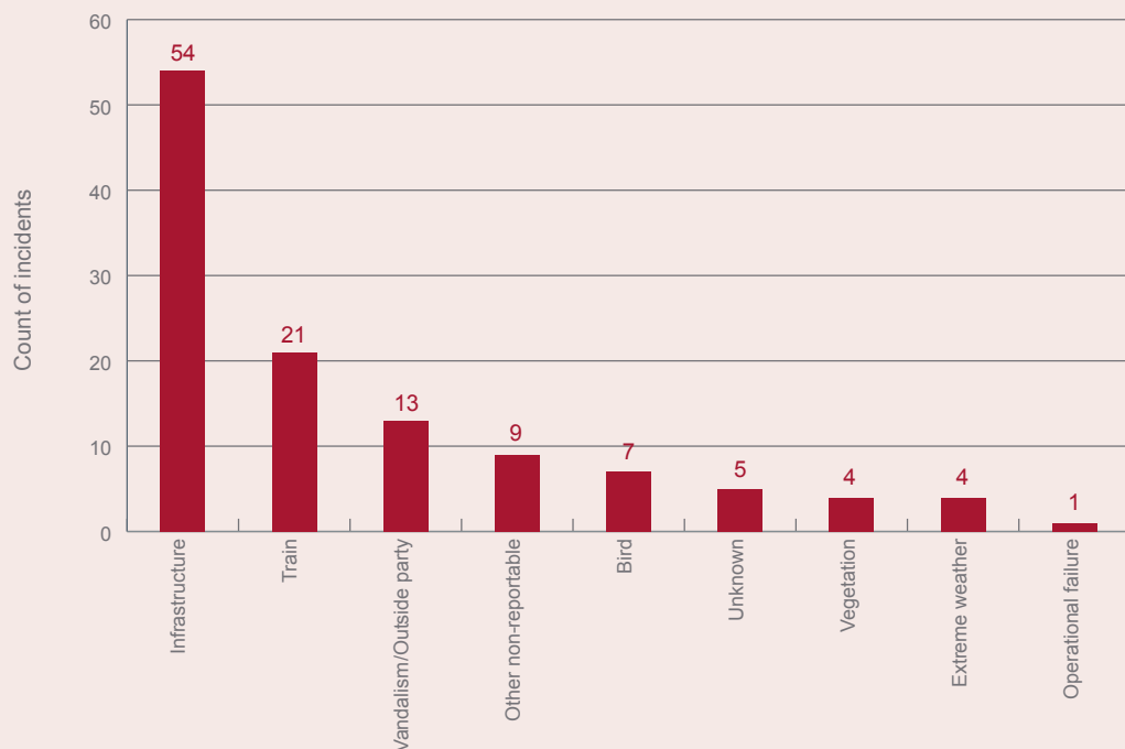
Figure 3.9 – AC traction power incidents 2007/08
