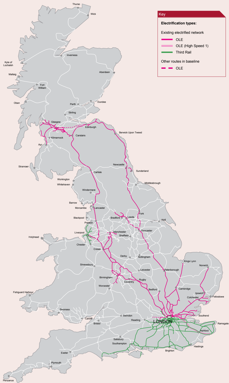
Figure 3.1 – Baseline: electrification types
