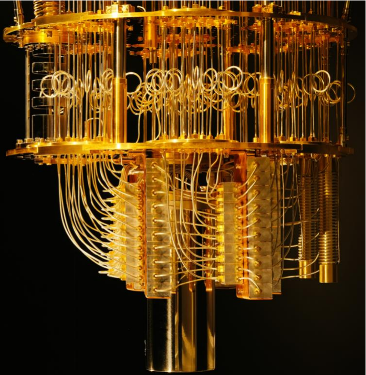
FIGURE 1: - IBM Quantum System Computer
